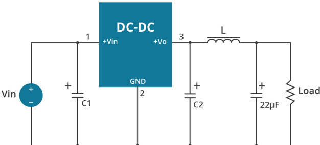
Positive Output Ripple Reduction Circuit
