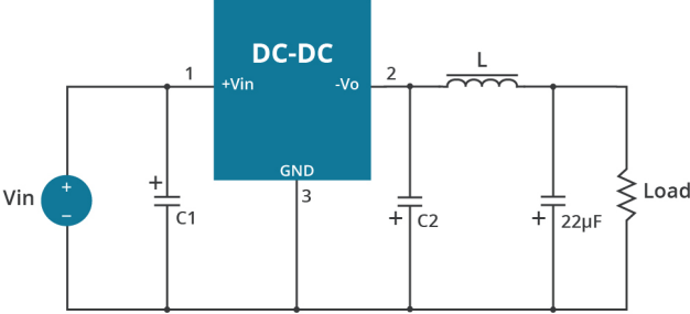
Negative Output Ripple Reduction Circuit
