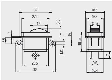
Screw connection chromated M3 without screw
