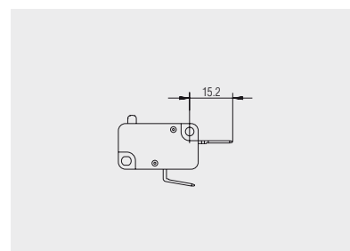
Quick-connect terminal 6.3 normally open contact version
