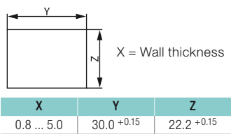
Basic types 1672, 1673 and 1675 single-pole illuminated / non-illuminated
