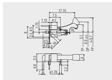
⌋ PCB terminal right angled 1010.9852
