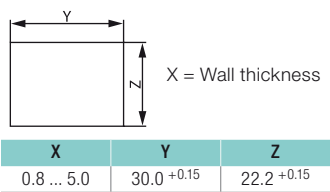
Basic types 1670 and 1671 double-pole illuminated / non-illuminated
