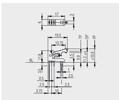
⌋ PCB terminal straight
