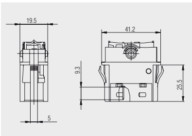
Quick-connect terminal 3.0 x 0.8
