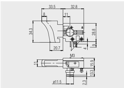
Socket terminal M3, terminal connection
