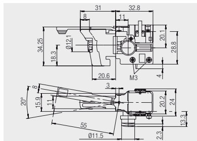
Socket terminal M3 mains side, screwless push-in terminal motor side, quick-connect terminal, 1298.7101
