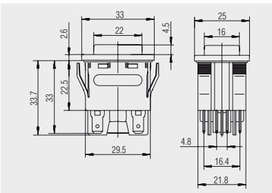
Quick-connect terminal 4.8 1673.5501
