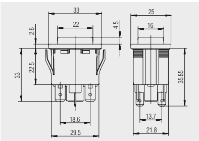
Quick-connect terminal 6.3 / 2 x 4.8 chromated external lamp connection 1670.5304
