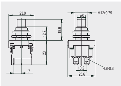
Quick-connect terminal 4.8
