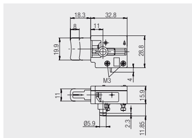
Socket terminal M3 mains side, screwless push-in terminal motor side 1298.0301
