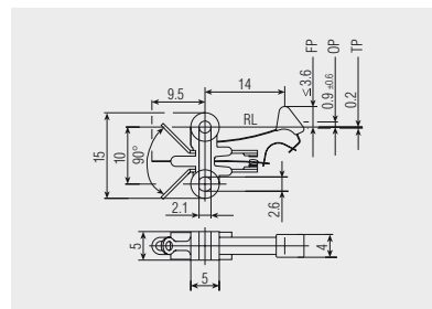
⌋ Solder terminal 45° angled 9.5 long
