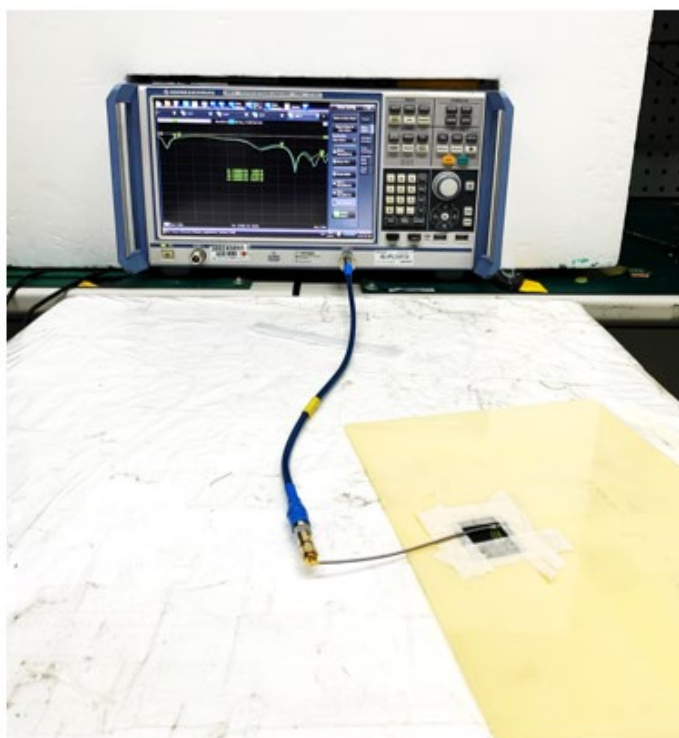
VNA Setup
