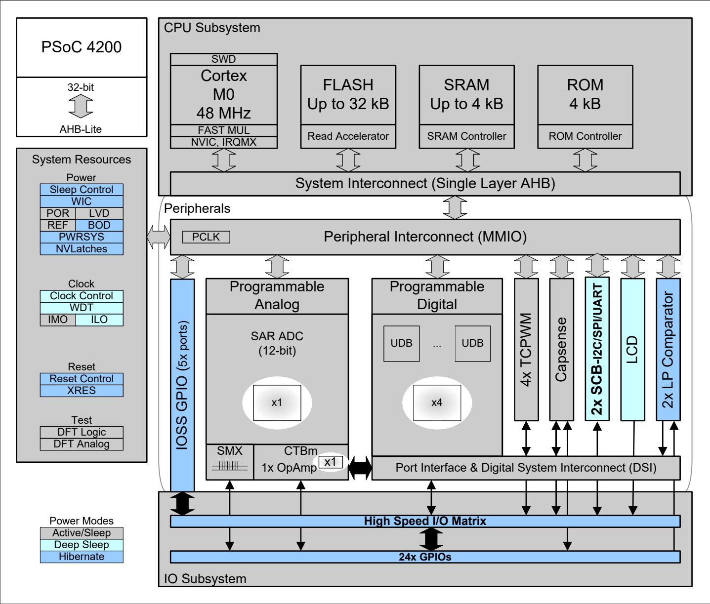
Figure 1 Block diagram
