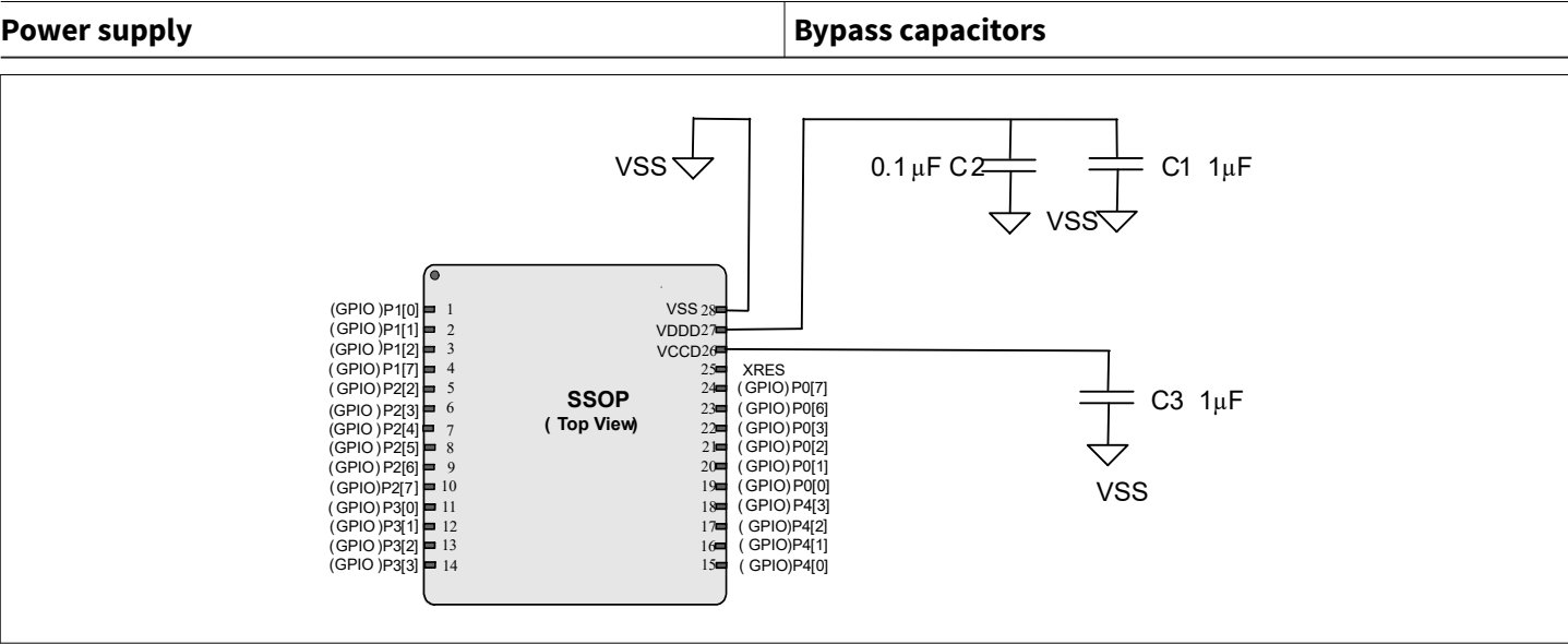
Figure 8 28-pin SSOP example
