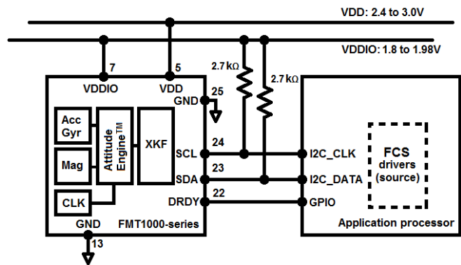
Figure 3. Typical Application
