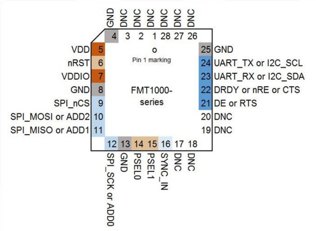
Figure 4. Pin Assignment
