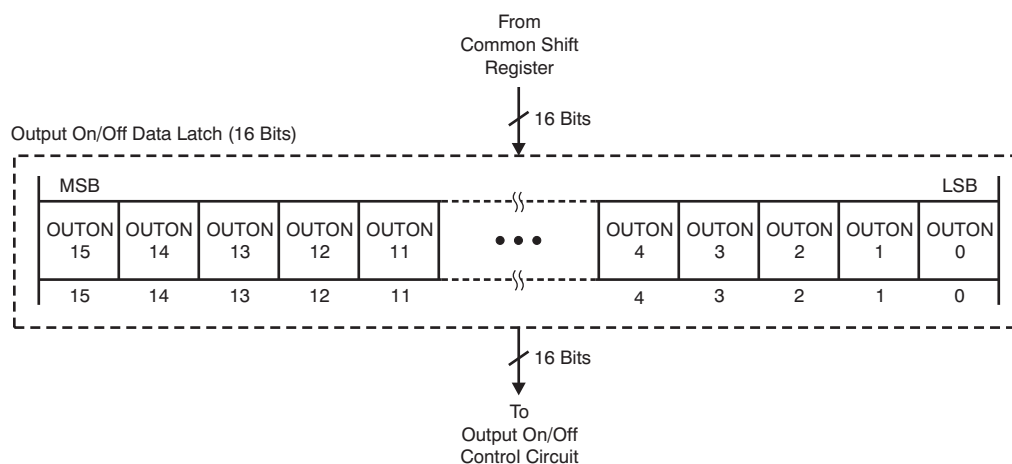
Figure 21. Output On/Off Data Latch Configuration
