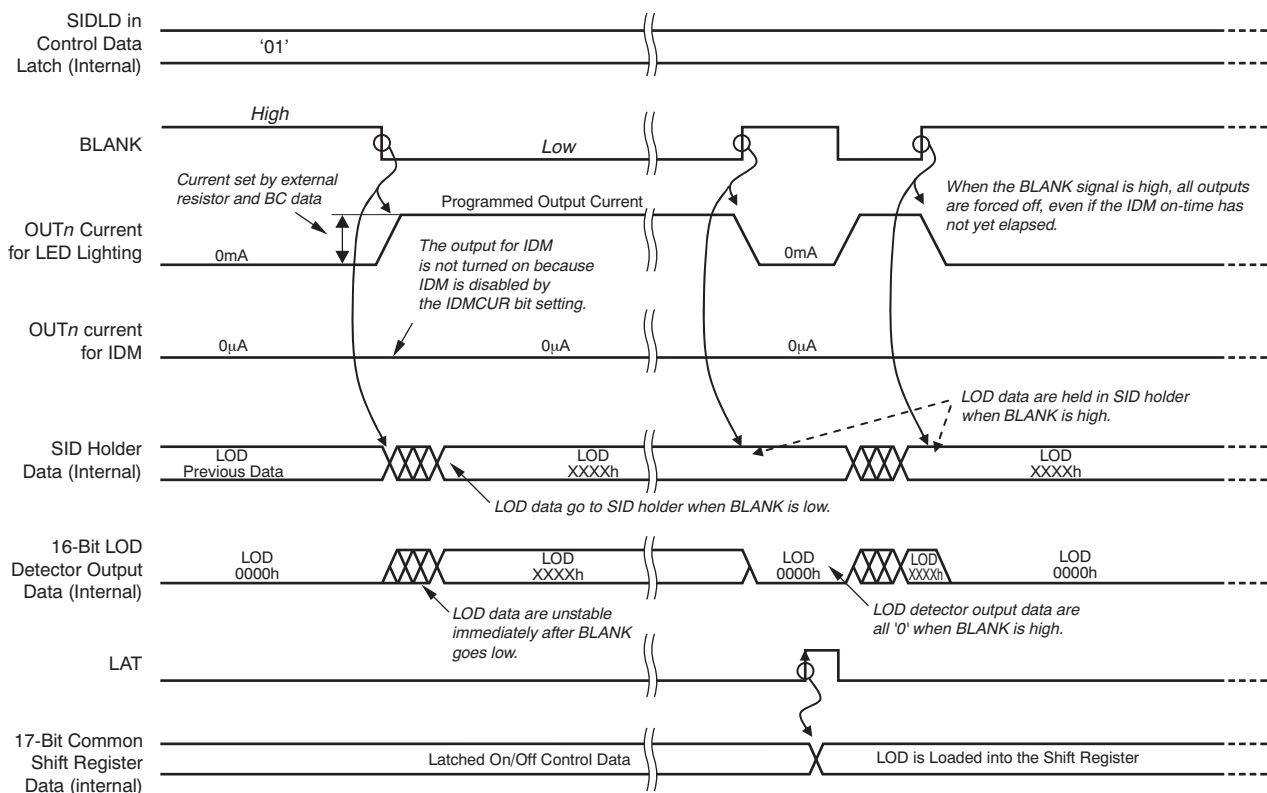
Figure 28. IDM Operation Timing with LOD Selected and IDM Disabled
