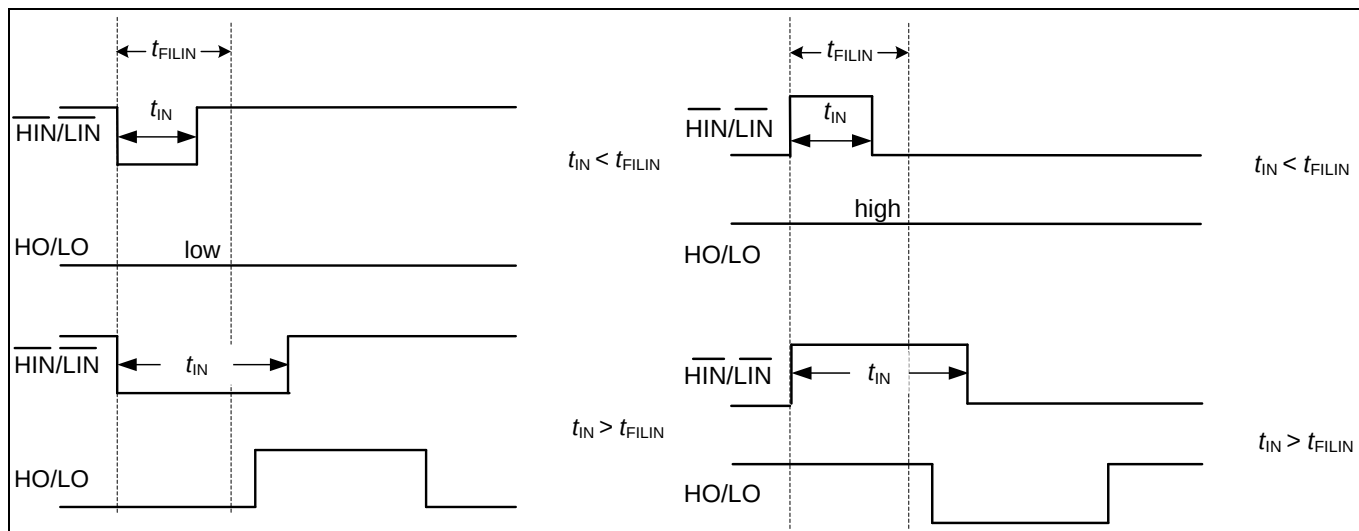
Figure 9 Timing of short pulse suppression (6EDL04I06NT)
