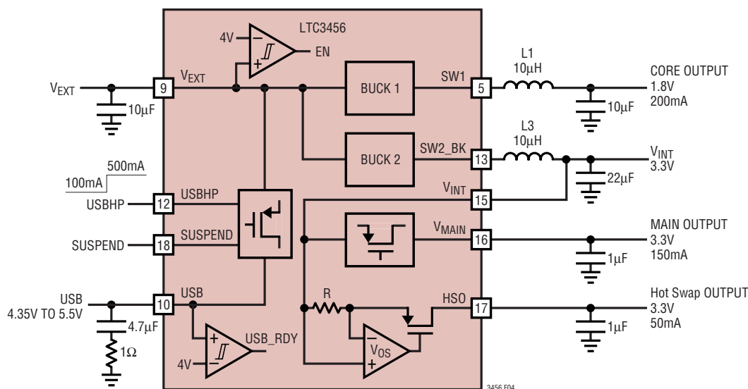
Figure 4. USB-Powered LTC3456
