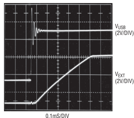
Figure 13(a). Hot-Plugging the USB Power (5.5V Input) with a 4.7μF Ceramic Capacitor Used for Bypassing.
