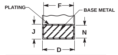
SECTION AE-AE
