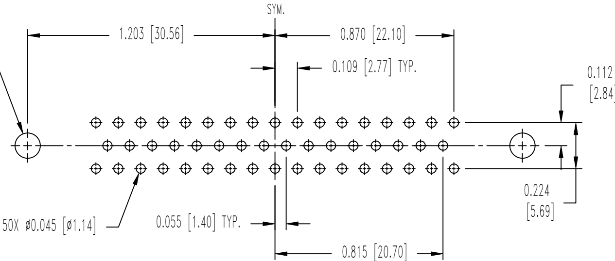
CONTACT HOLE PATTERN
