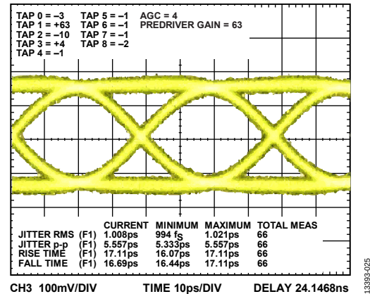
Figure 26. Typical Output Waveform at 25.8 Gbps, PRBS 2^{31} - 1 Input Data
