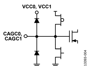
Figure 5. CAGCx Interface Schematic
