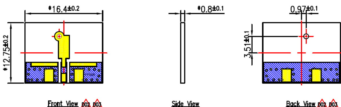
Evaluation Board
