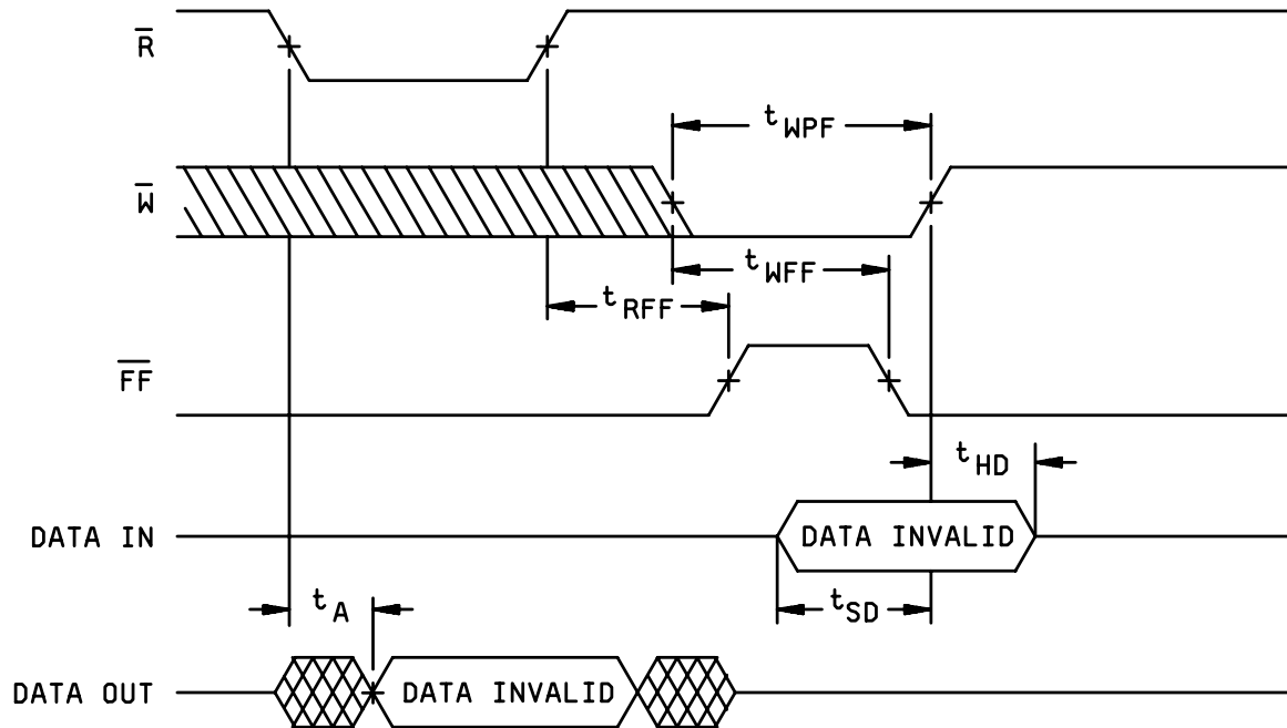
FULL FLAG AND WRITE BUBBLE-THROUGH MODE TIMING DIAGRAM
