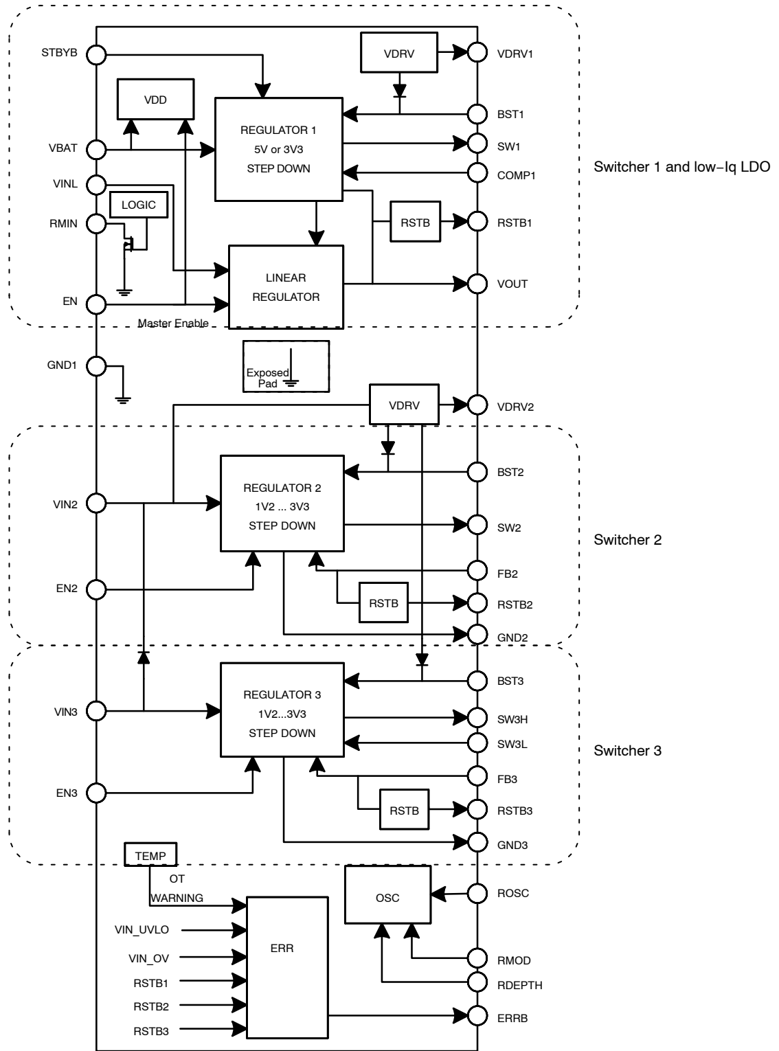
Figure 24. NCV97311 Block Schematic
