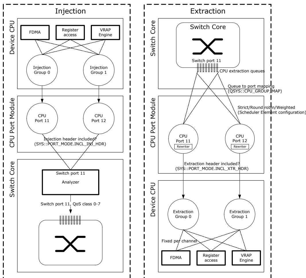
FIGURE 2-38: CPU INJECTION AND EXTRACTION
