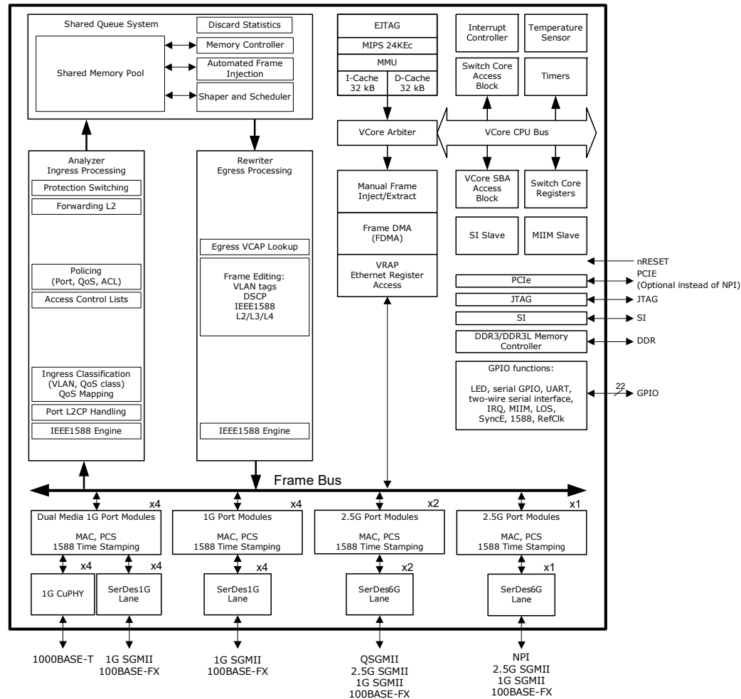
FIGURE 1-1: BLOCK DIAGRAM
