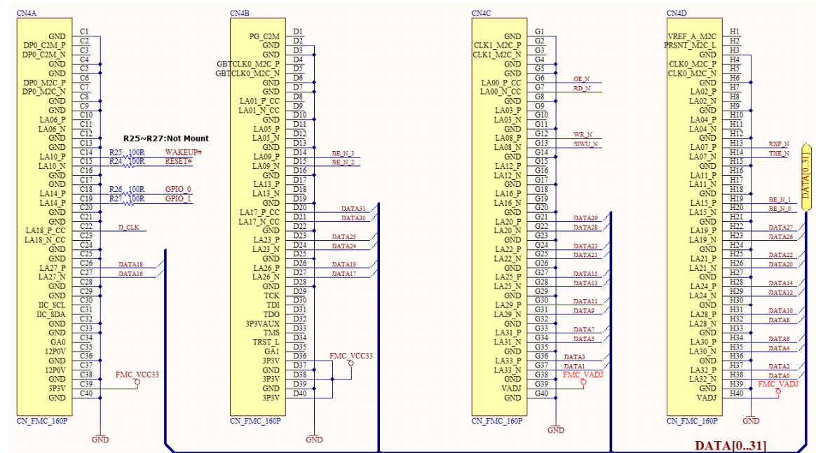
Figure 3-7 Schematics: FMC_UMFT601X
