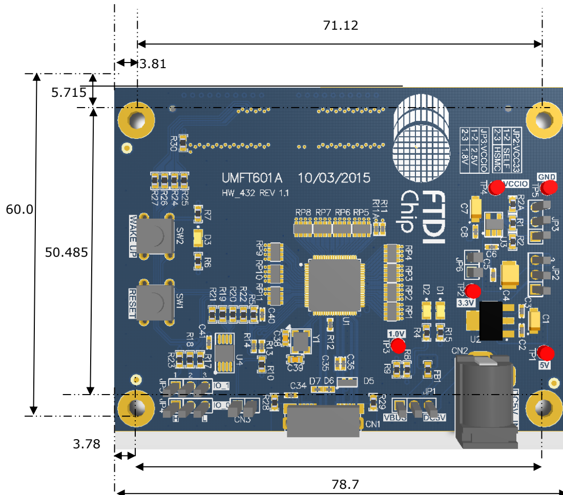
Figure 2-5 UMFT600A/UMFT601A Dimensions (Top view)
