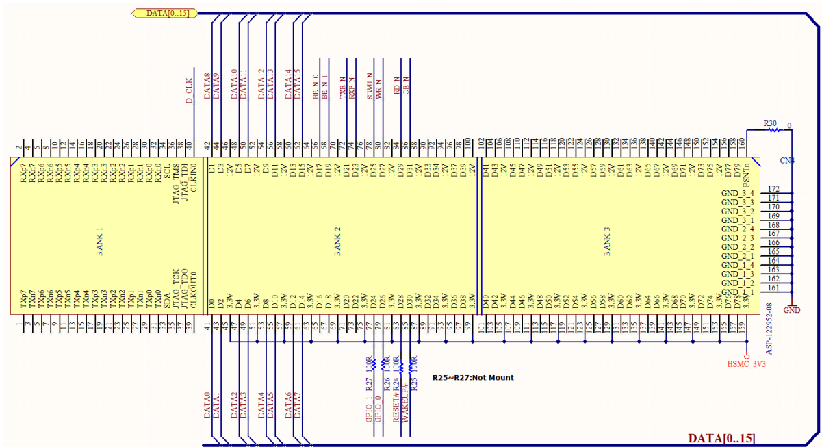
Figure 3-4 Schematics: HSMC_UMFT600A
