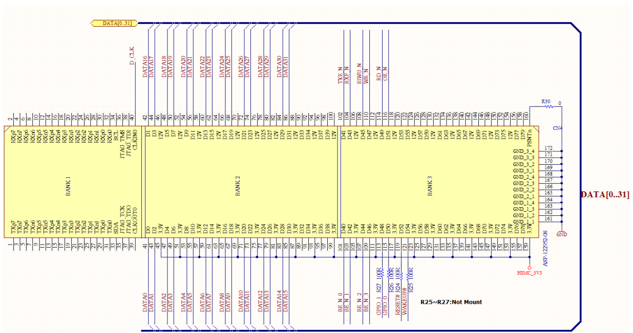
Figure 3-5 Schematics: HSMC_UMFT601A
