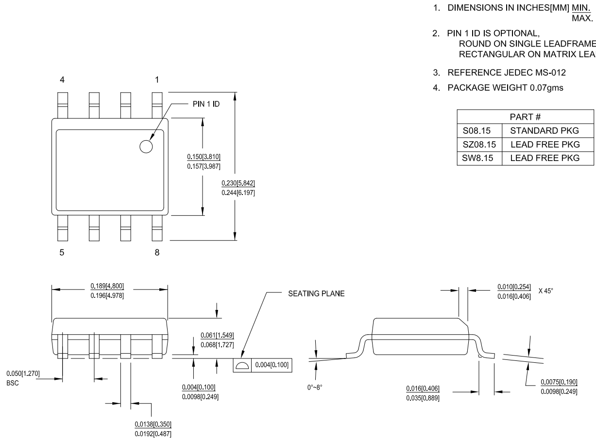
Figure 20. 8-pin SOIC (150 Mils) Package Outline, 51-85066
