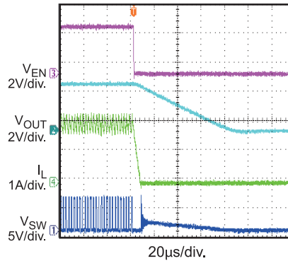
Shutdown Through EN I_{OUT} = 2A
