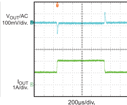
Load Transient I_{OUT} = 1A \leftrightarrow 2A , 1.6A/\mu s
