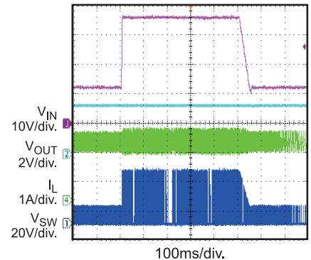
Load Dump V_{IN} = 12V \leftrightarrow 36V , I_{OUT} = 2A
