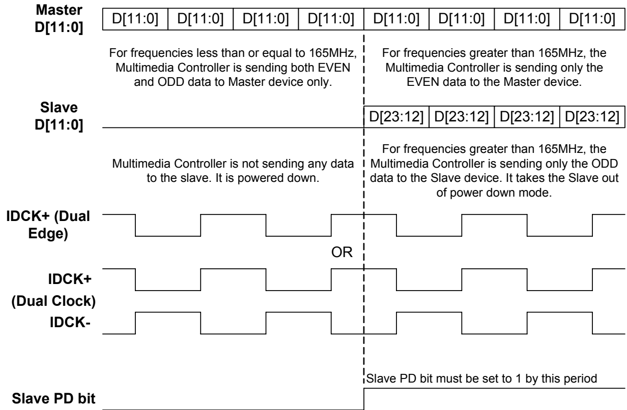
Figure 16. Single/Dual Link Timing Diagram
