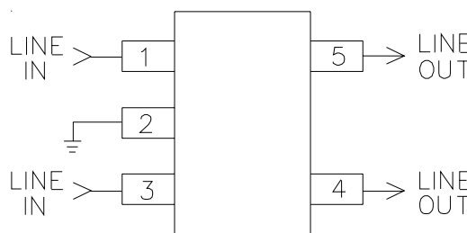
Figure 2 - STF701 Connection Diagram
