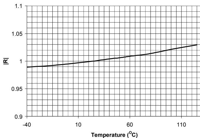
Normalized Resistance vs. Temperature
