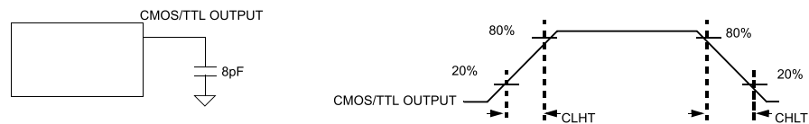
Figure 6. RHFLVDS218 output load and transition times
