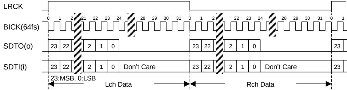
Figure 26. Mode 3/8 Timing (Stereo Mode)
