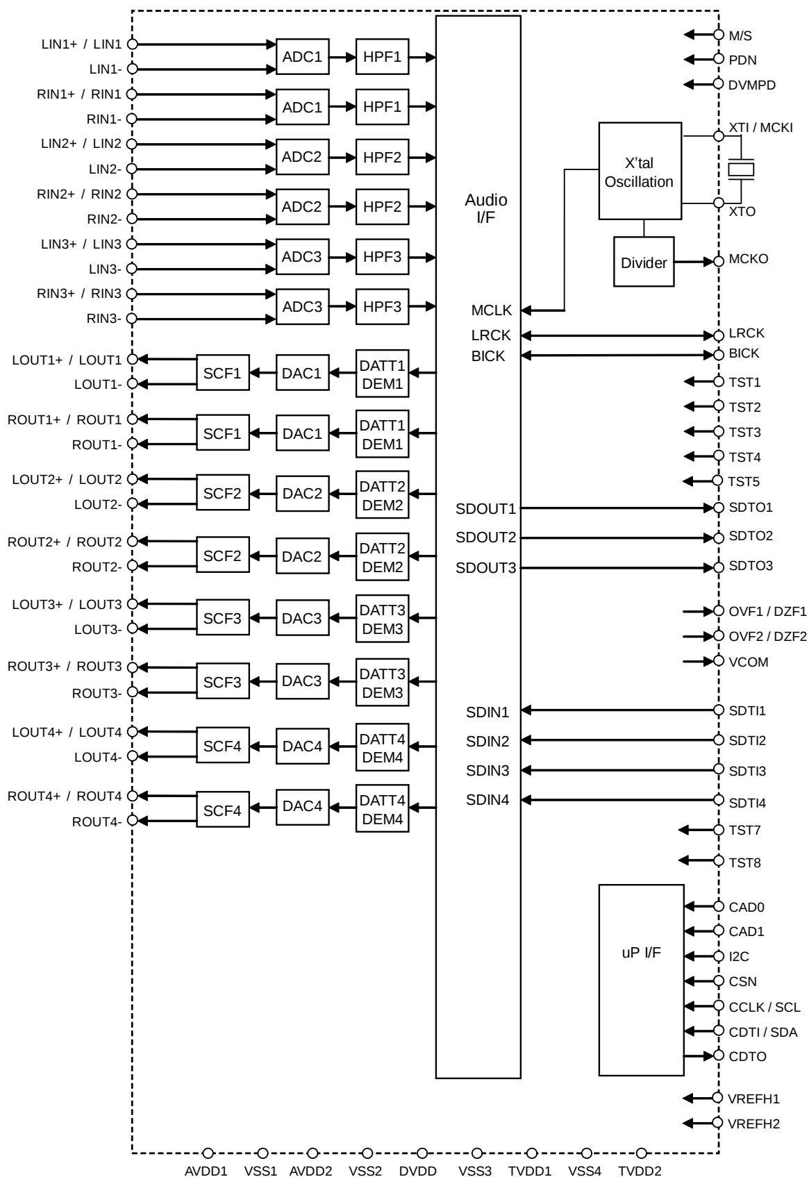
Figure 1. Block Diagram
