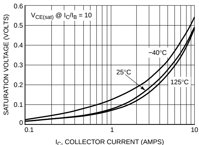
Figure 6. D45VH10 ON-Voltage
