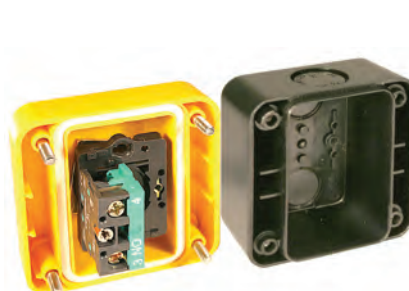
S3 Normally Open Gold plated
