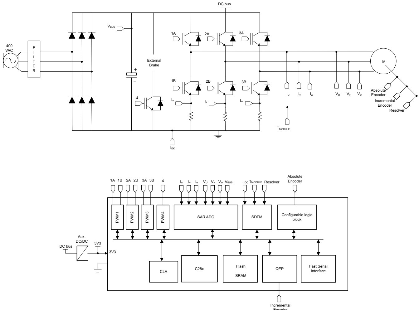
Figure 9-7. Servo Drive Control Module
