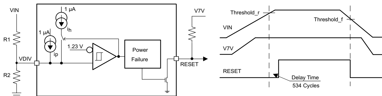
Figure 7-2. Power Failure Detector Timing Diagram
