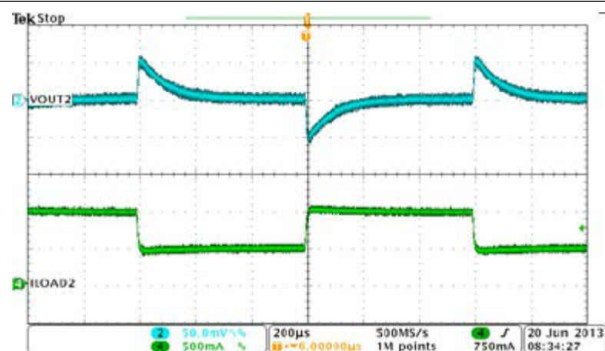
Figure 8-17. BUCK2, Load Transient, 0.5 A to 1.0 A SR = 0.25 \text{ A}/\mu\text{s}
