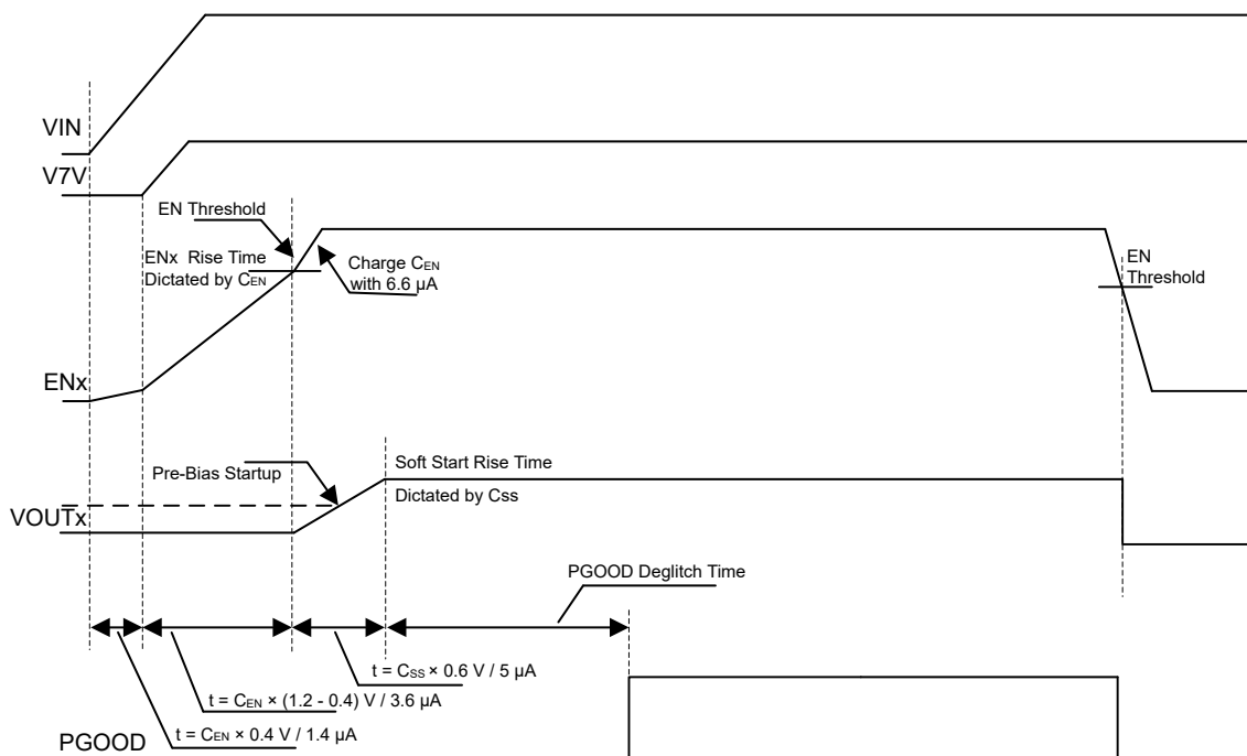
Figure 7-8. Startup Power Sequence
