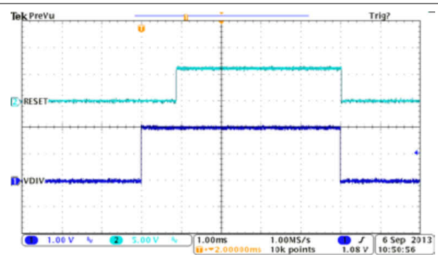
Figure 8-34. Deglitch Time, Reset vs VDIV
