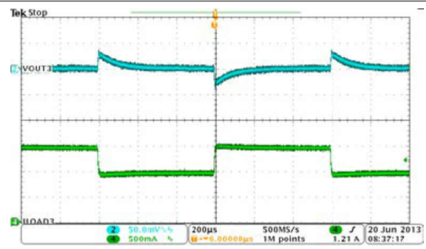
Figure 8-20. BUCK3, Load Transient, 1.0 A to 1.5 A SR = 0.25 \text{ A}/\mu\text{s}
