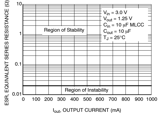
Figure 13. Typical ESR vs. Output Current
