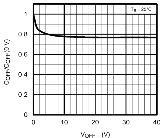
Fig. 12.1.11 C_{OFF}/C_{OFF}(0V) - V_{OFF}
