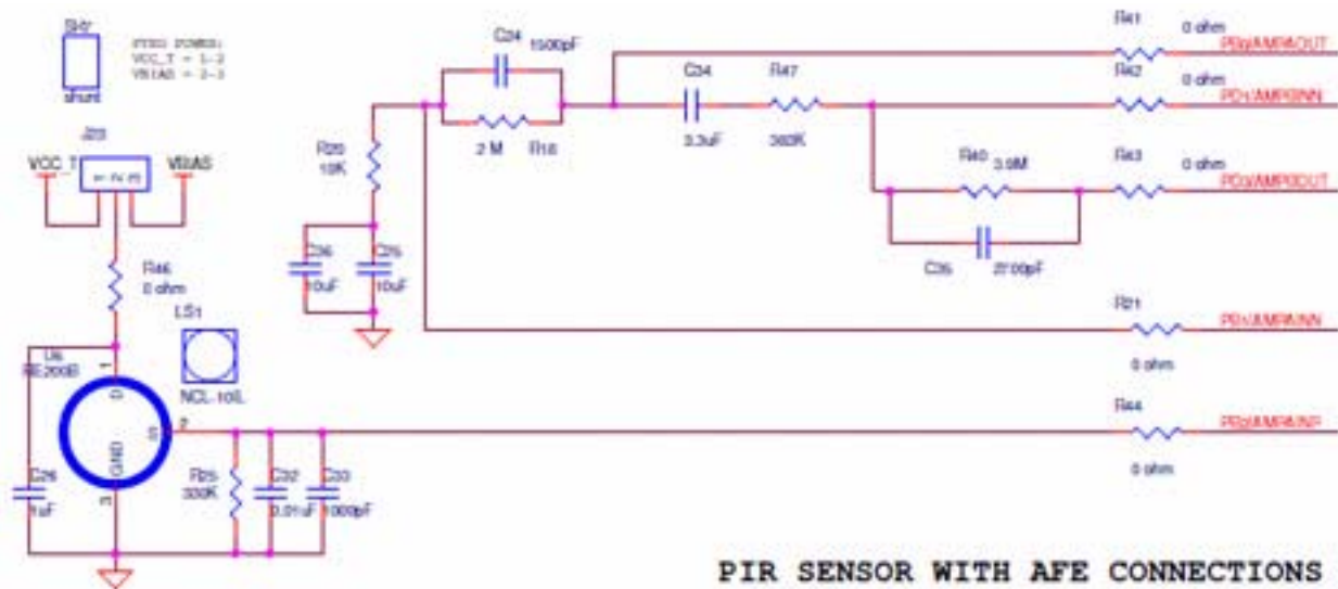
Figure 23. RE200B Pyroelectric Sensor Circuit
