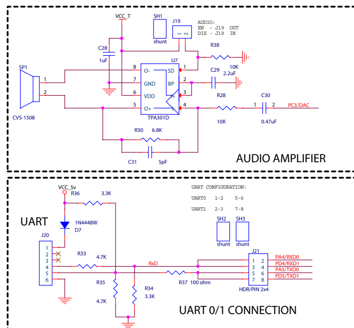
Figure 40. F6482 Series Development Board Schematic Diagram, #4 of 4
