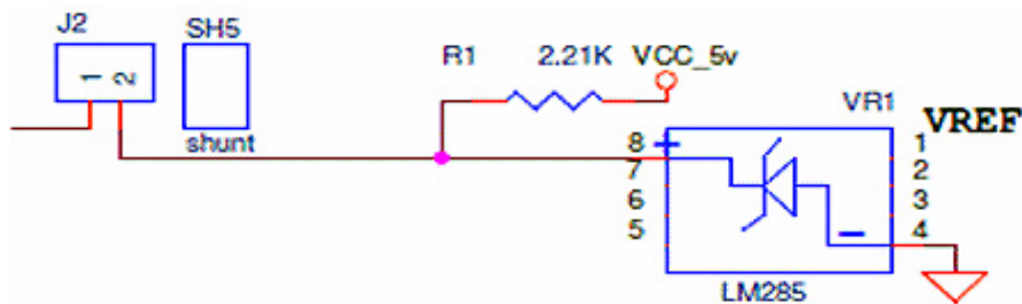
Figure 32. LM285 Adjustable Micropower Circuit
