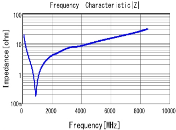
■ GRM1555C1H820GA01 |Z| DC0V, 25degC
