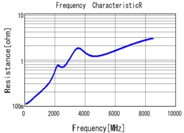
■ GRM1555C1H820GA01 R DC0V, 25degC
