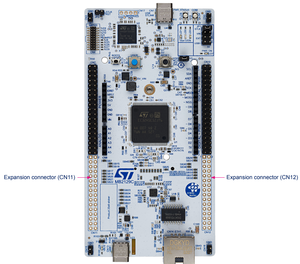
Figure 16. Expansion connectors
