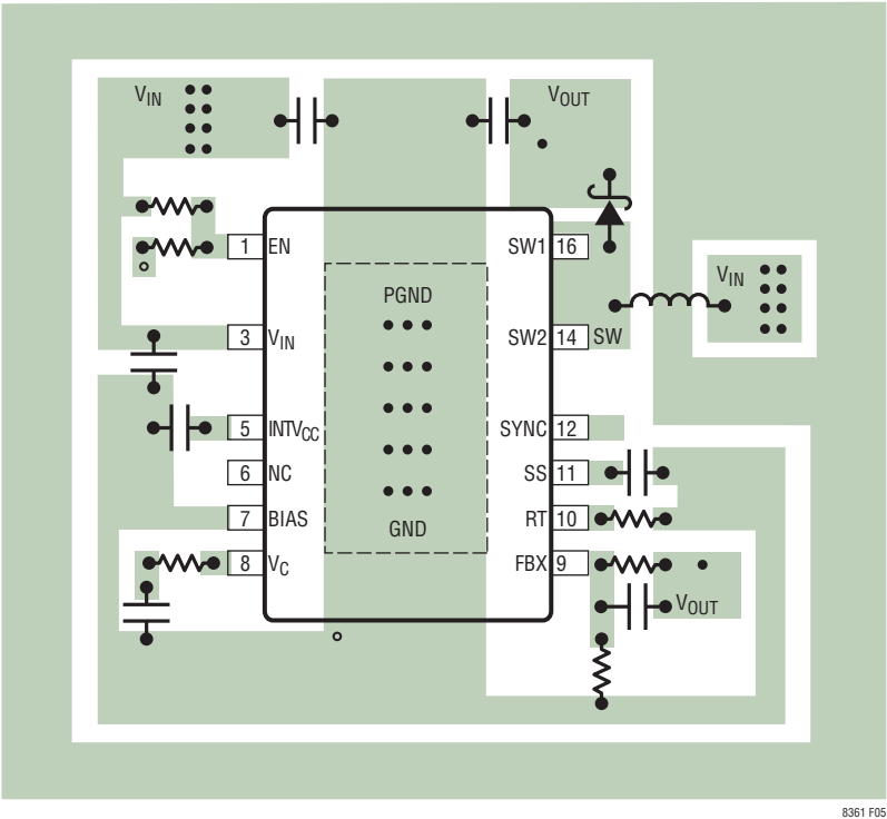
Figure 5. Suggested Boost Converter Layout
