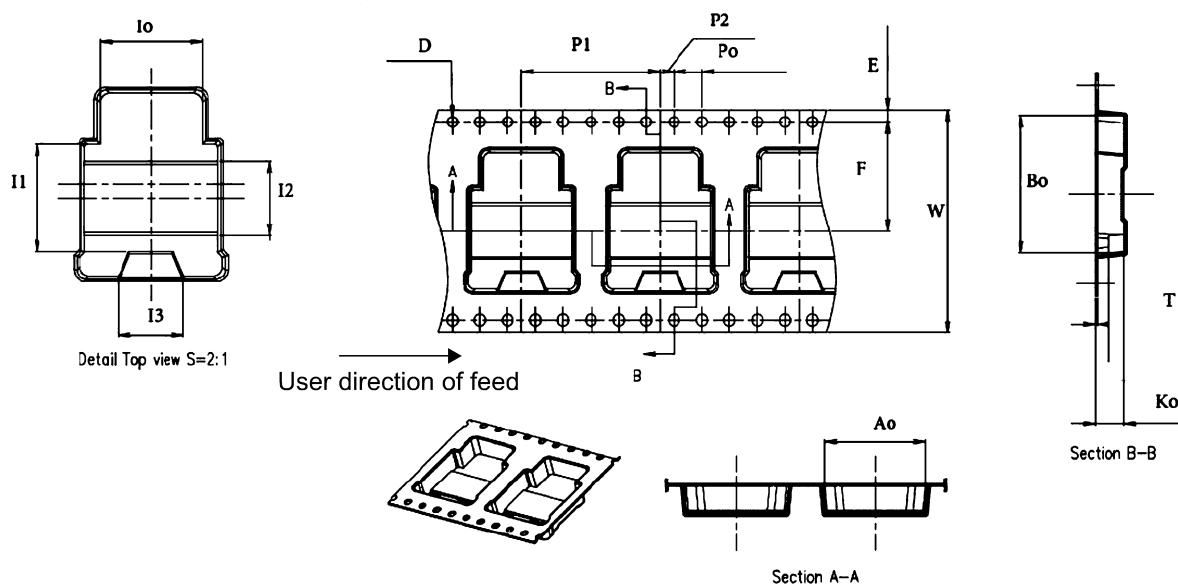
Figure 18. HU3PAK carrier tape outline
