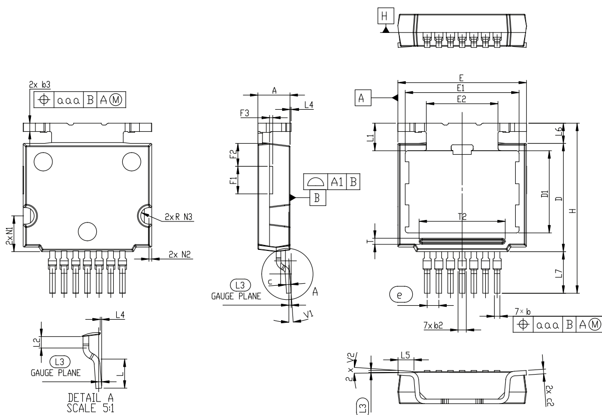
Figure 16. HU3PAK package outline
