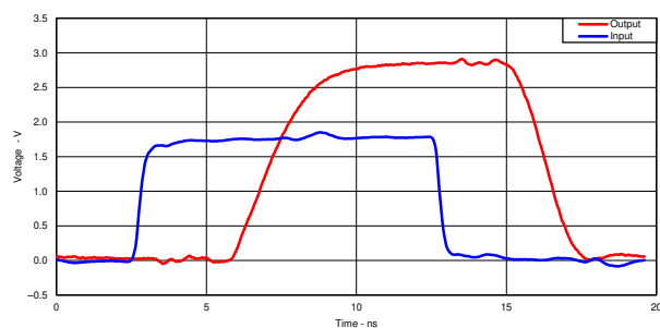
Figure 7-1. Switching Characteristics at 50 MHz Excellent Signal Integrity (1.8 V to 3.3 V at 3.3-V V_{CC} )
