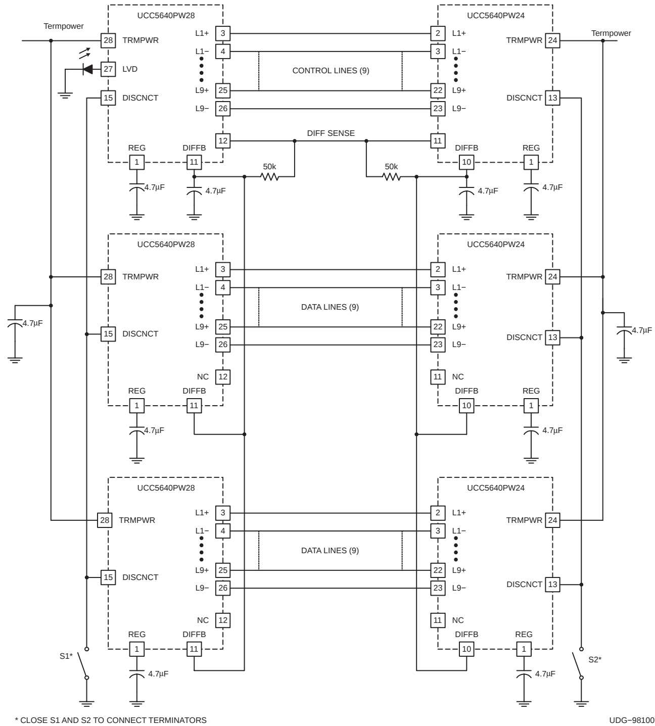
Figure 1. Application Diagram
