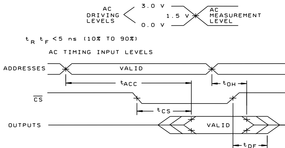
FIGURE 4. AC read timing diagram.
