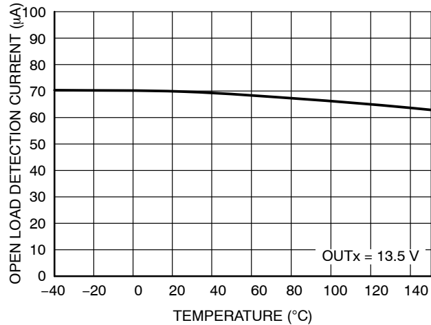
Figure 16. Output Load Detection Current vs. Temperature
