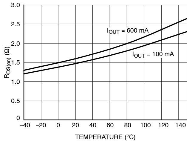
Figure 12. Output R DS(on) vs. Temperature
