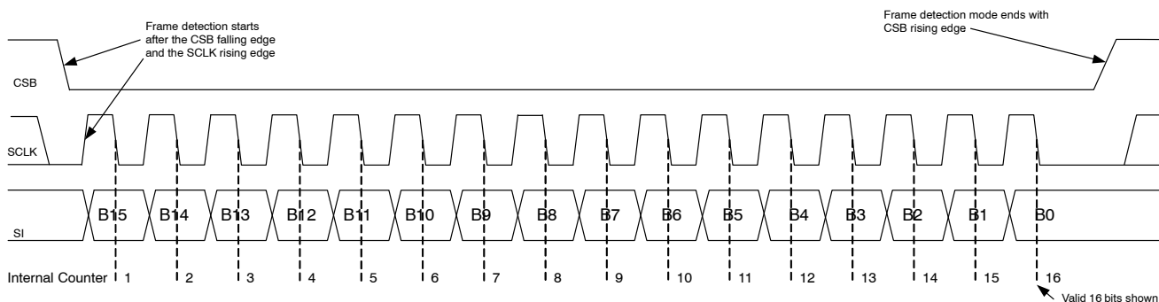
Figure 30. Frame Detection
