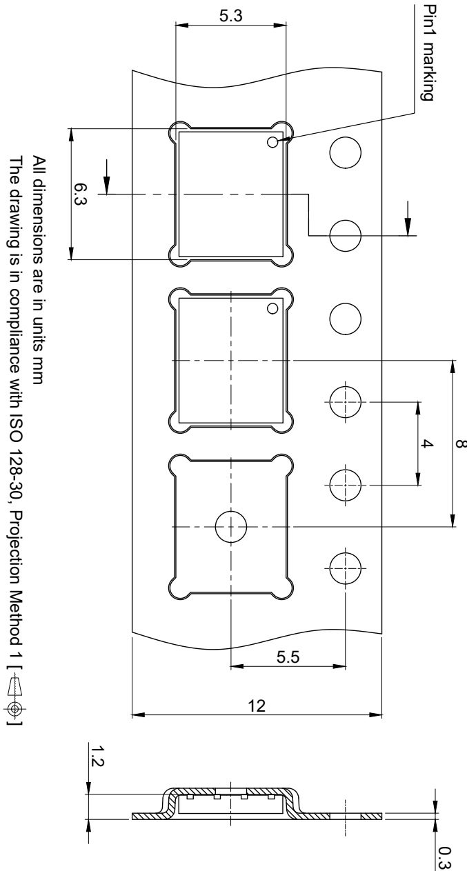
Figure 3 Packaging variant PG-TSON-8, dimensions in mm
