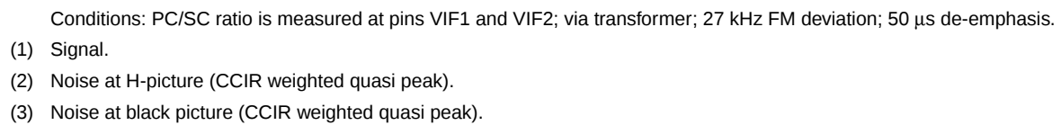
Fig 18. Audio signal-to-noise ratio as a function of picture-to-sound carrier ratio in intercarrier mode.
