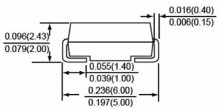
SMB/DO-214AA
