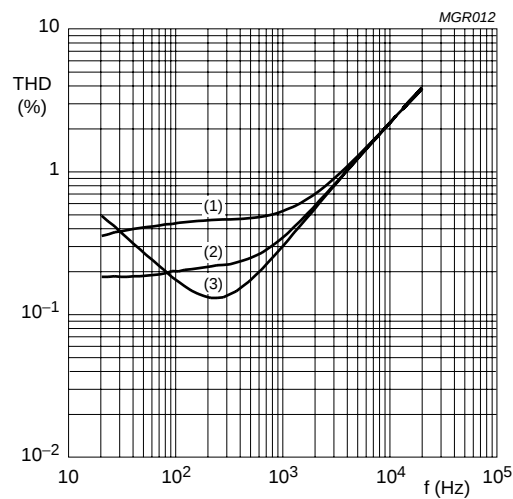
V_{DD} = 5\text{ V} ; R_L = 8\ \Omega ; P_O = 0.1\text{ W} ; G_V = 30\text{ dB (max.)} . (1) G_V = 0\text{ dB} . (2) G_V = 7\text{ dB} . (3) G_V = 30\text{ dB} .
