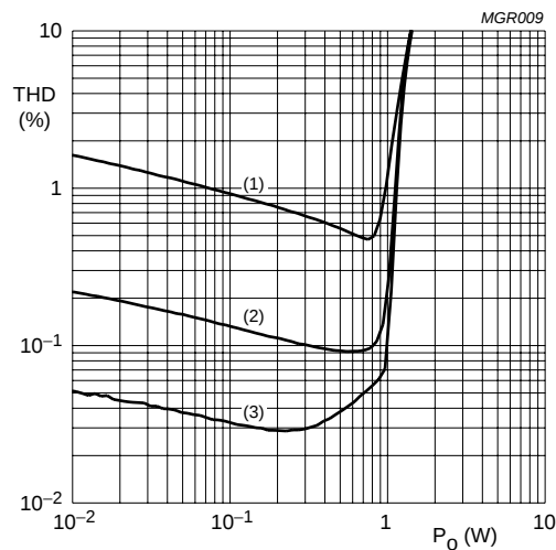
V_{DD} = 5\text{ V} ; R_L = 8\ \Omega ; G_V = 20\text{ dB (max.)} . (1) f = 10\text{ kHz} . (2) f = 1\text{ kHz} . (3) f = 100\text{ Hz} .
