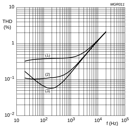
V_{DD} = 5\text{ V} ; R_L = 8\ \Omega ; P_O = 0.1\text{ W} ; G_V = 20\text{ dB (max.)} . (1) G_V = 0\text{ dB} . (2) G_V = 7\text{ dB} . (3) G_V = 20\text{ dB} .
