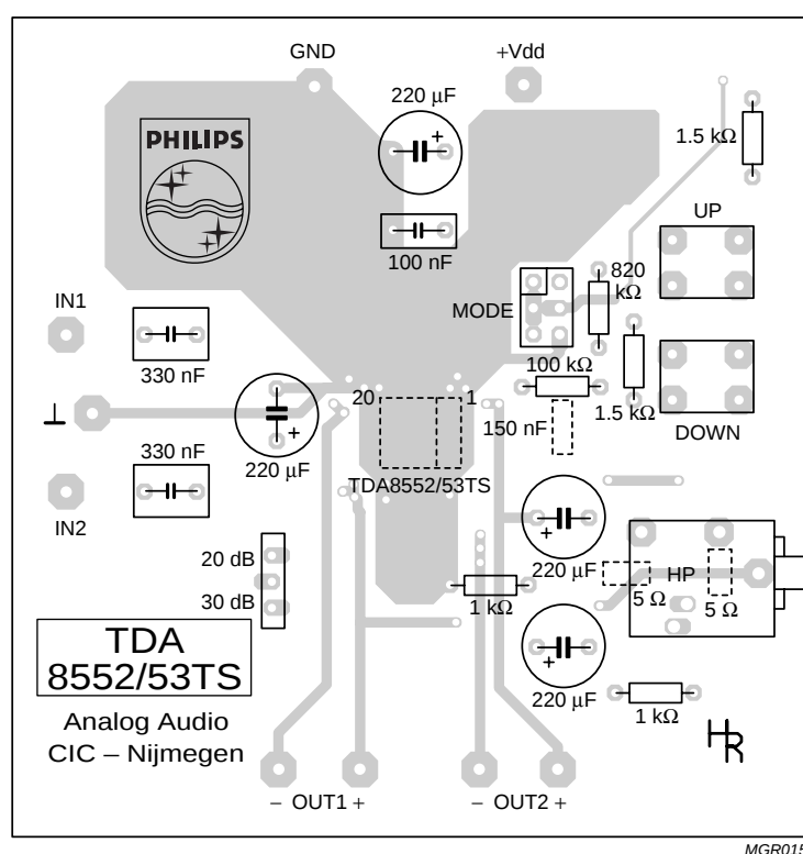
Fig.18 Printed-circuit board layout.
