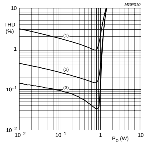
V_{DD} = 5\text{ V} ; R_L = 8\ \Omega ; G_V = 30\text{ dB (max.)} . (1) f = 10\text{ kHz} . (2) f = 1\text{ kHz} . (3) f = 100\text{ Hz} .
