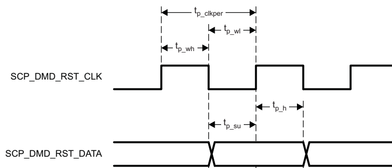
Figure 10. DLPA200 I/F Timing
