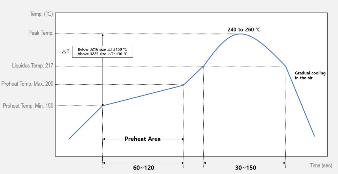
[Reflow Soldering Conditions]
