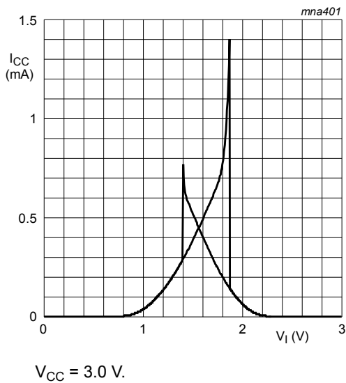
Fig. 10. Typical 74AHC3G14 transfer characteristics
