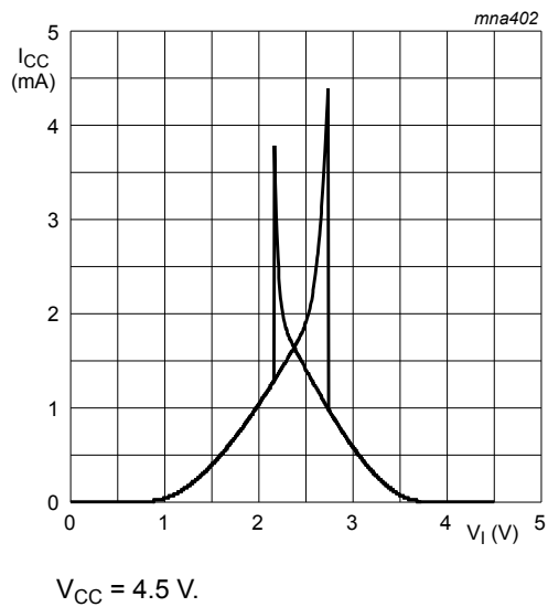
Fig. 11. Typical 74AHC3G14 transfer characteristics
