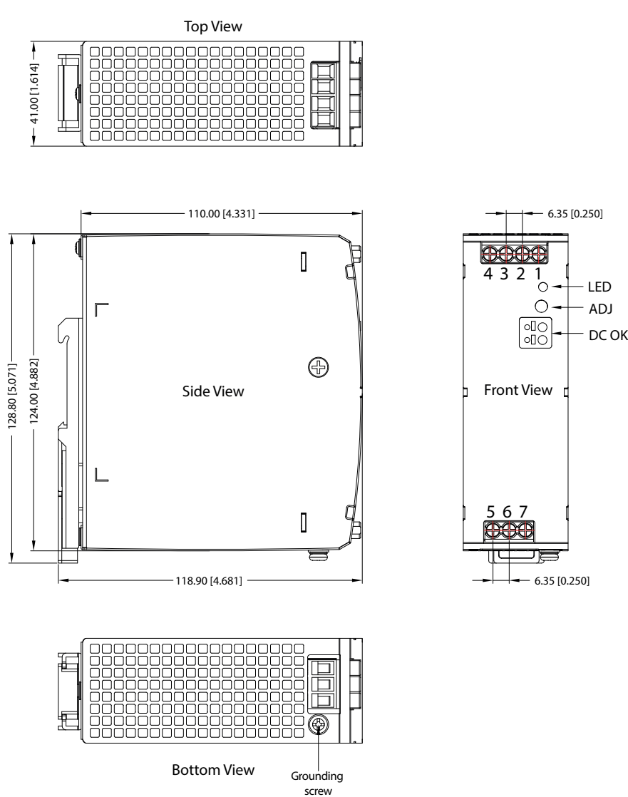
Figure 5. Mechanical Drawing
