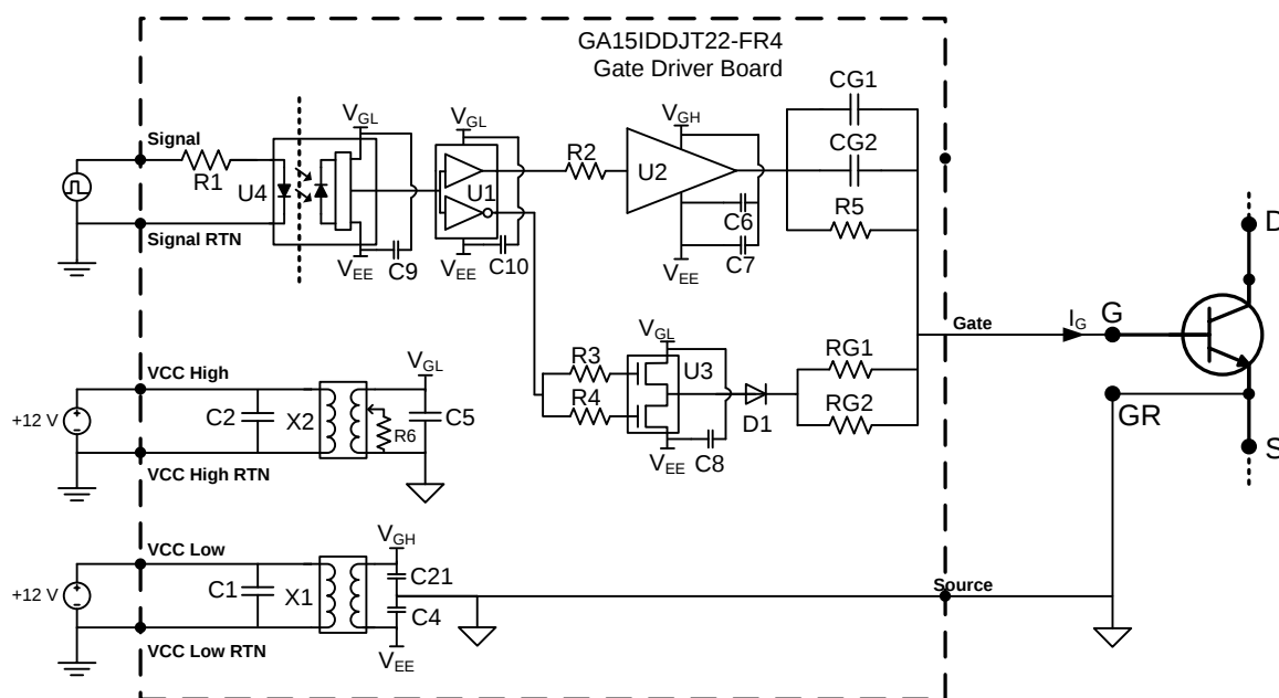
Figure 24: Topology of the GA15IDDJT22-FR4 Two Voltage Source gate driver.
