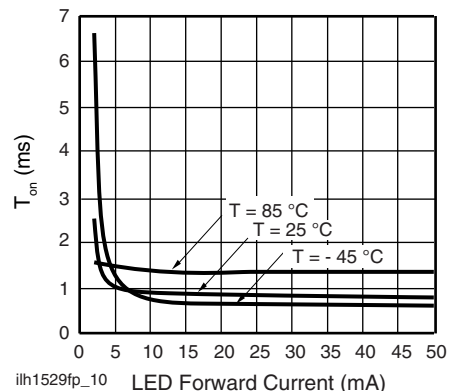
Fig. 10 - Turn-on Time vs. LED Current
