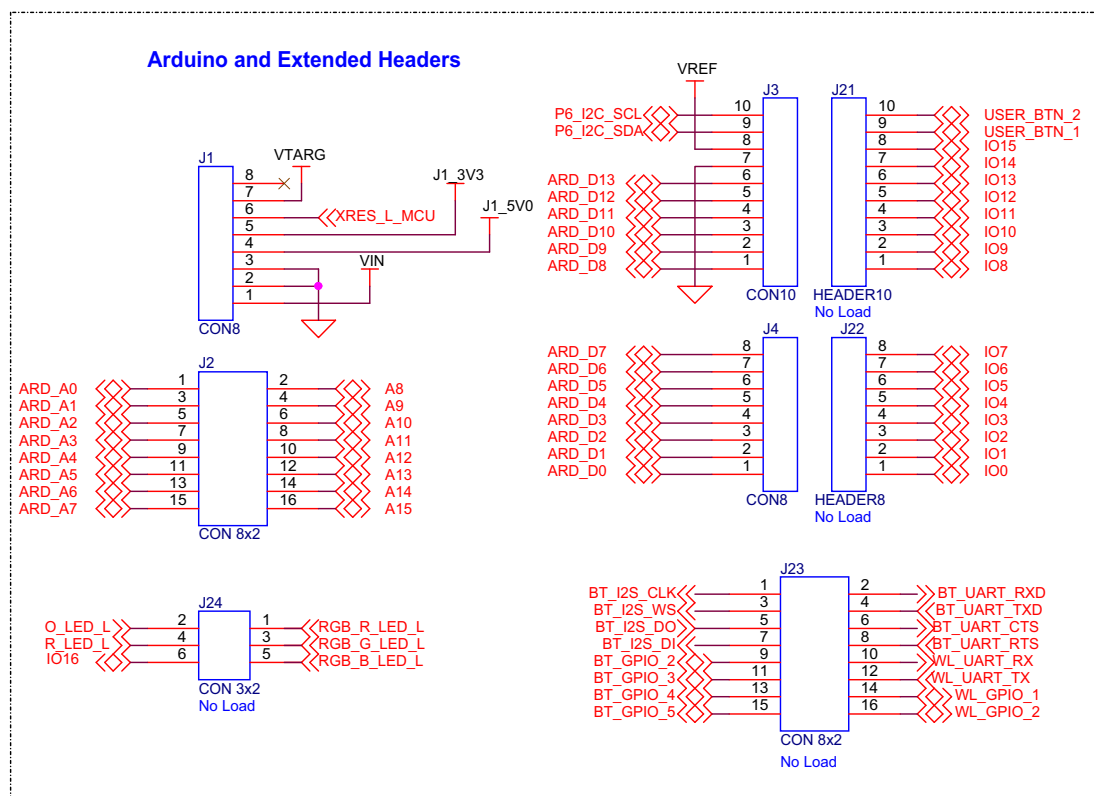
Figure 5-10. I/O Headers
