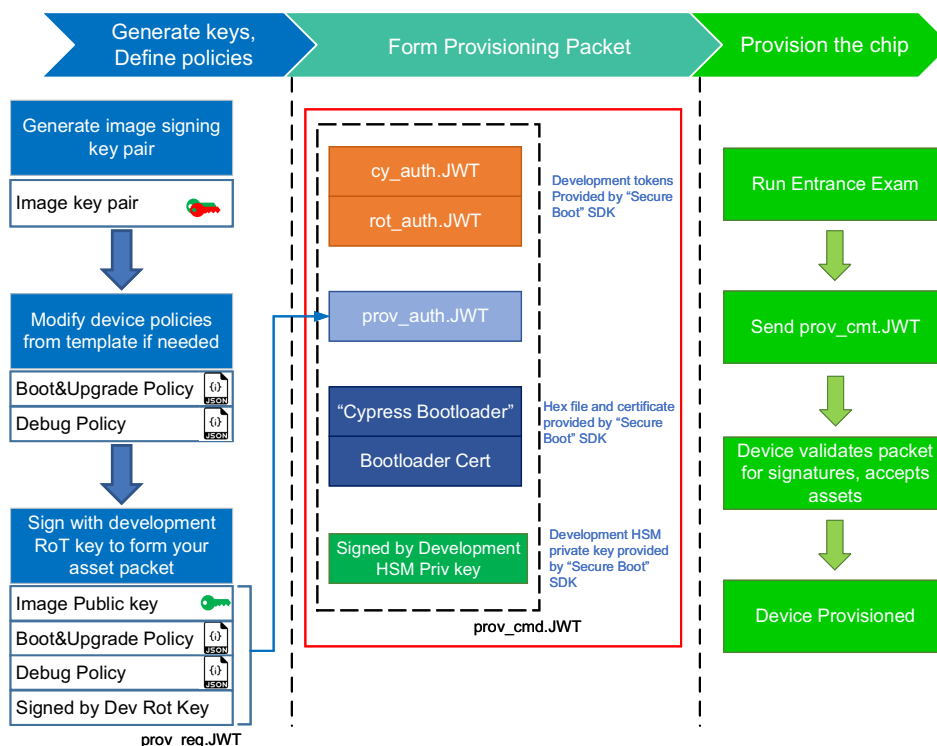
Figure 4-1. Provisioning Flow
