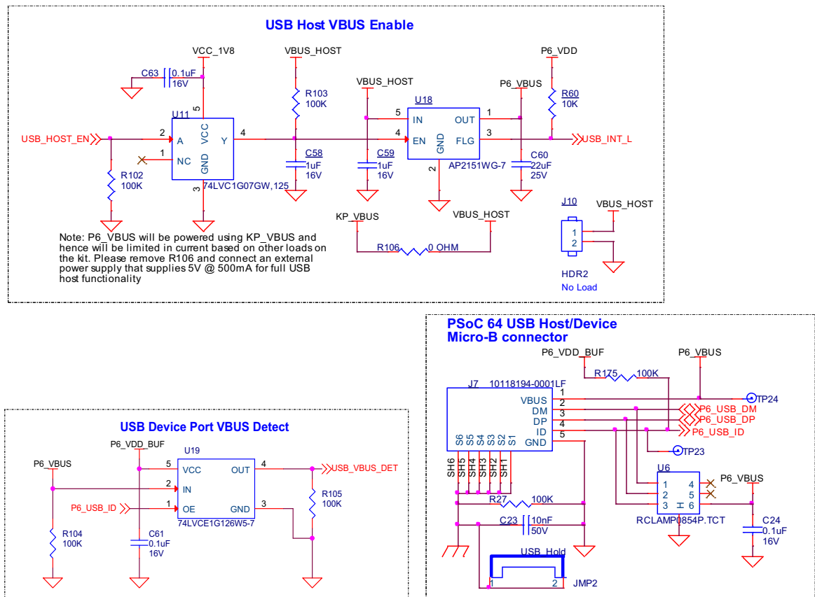
Figure 5-17. PSoC 64 USB
