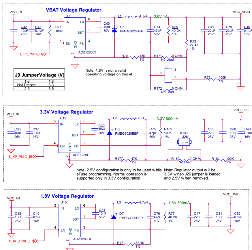
Figure 5-6. Voltage Regulators
