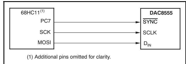
Figure 52. DAC8555 to 68HC11 Interface
