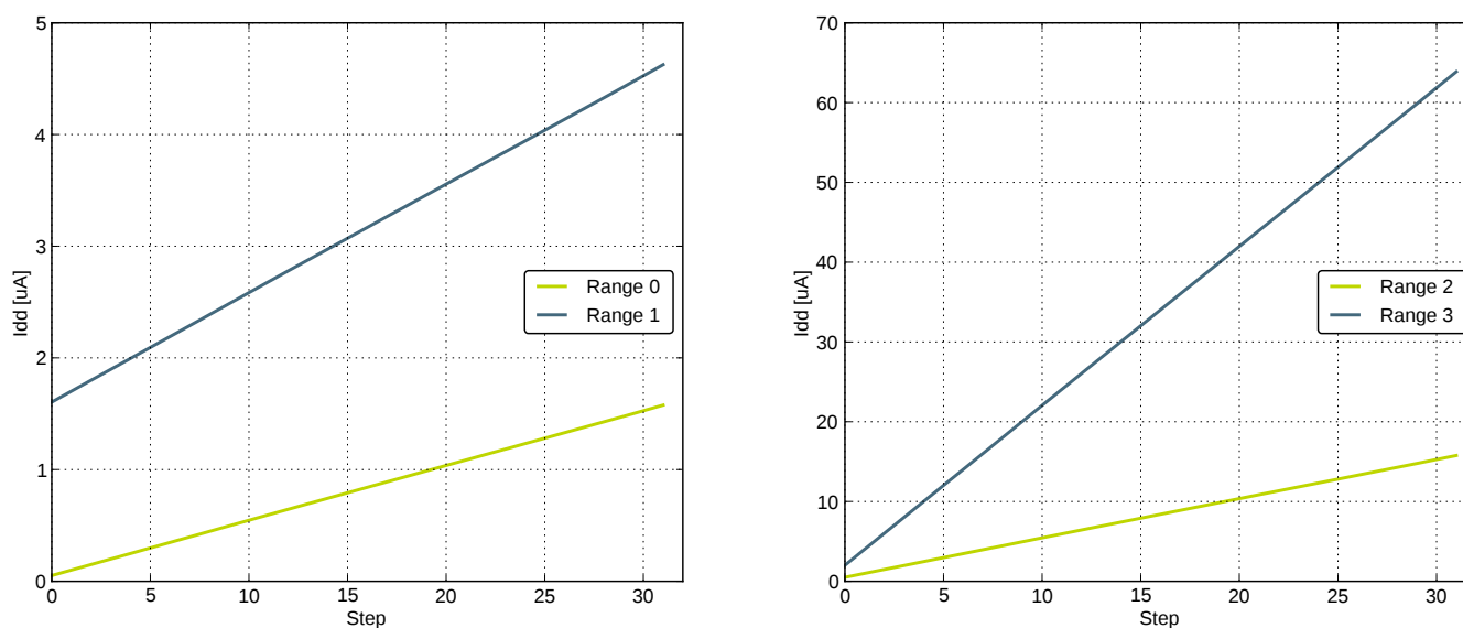
Figure 4.37. IDAC Linearity
